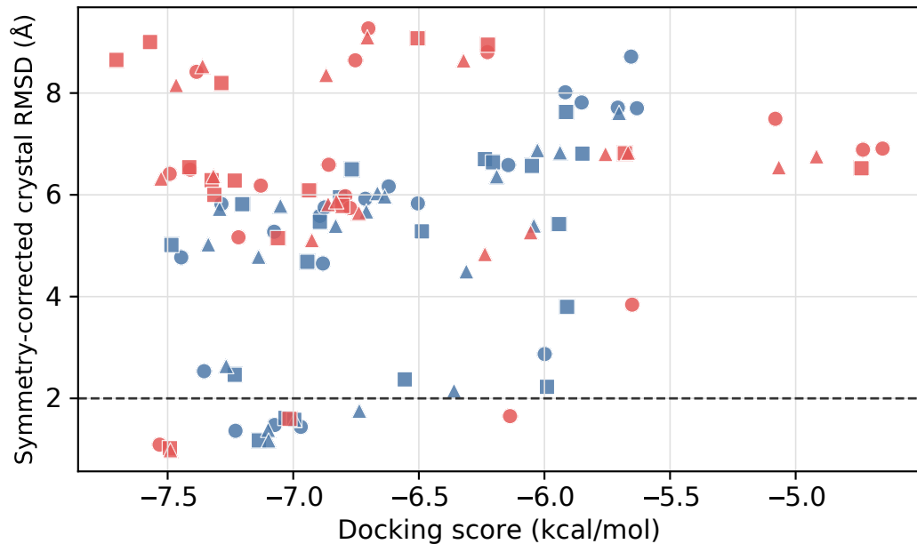
Score does not uniquely determine pose recovery
