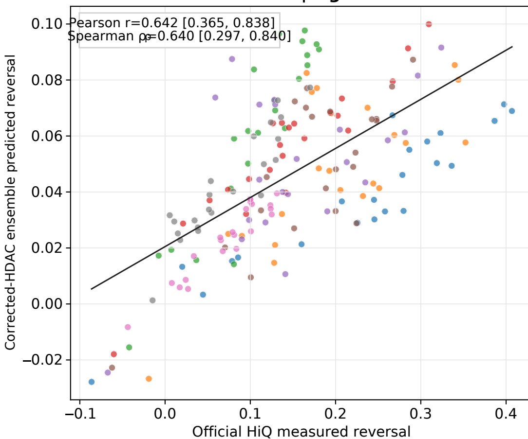
Dual stream | spearman reversal
