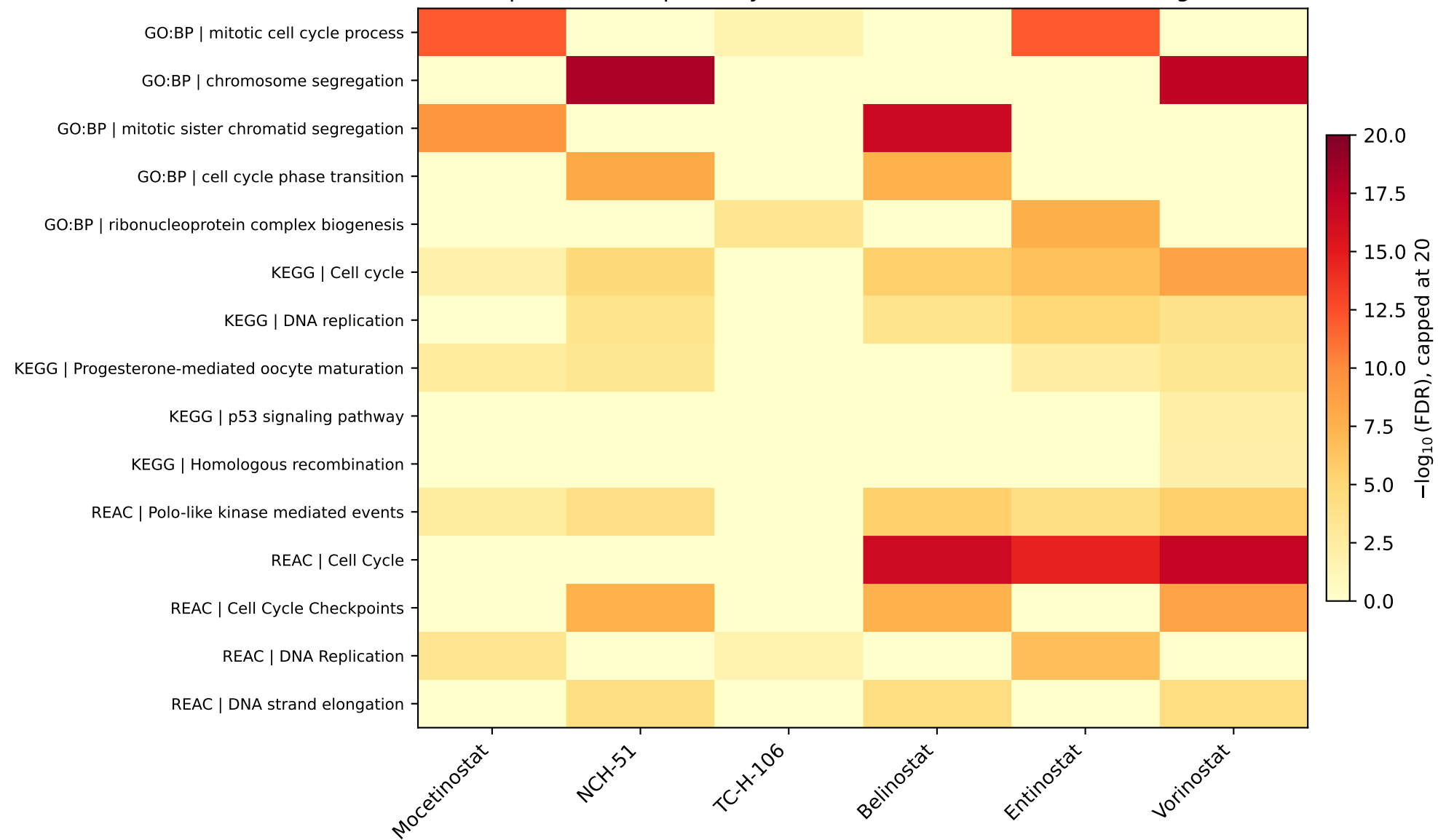
Representative pathway enrichment of reversal-associated genes
