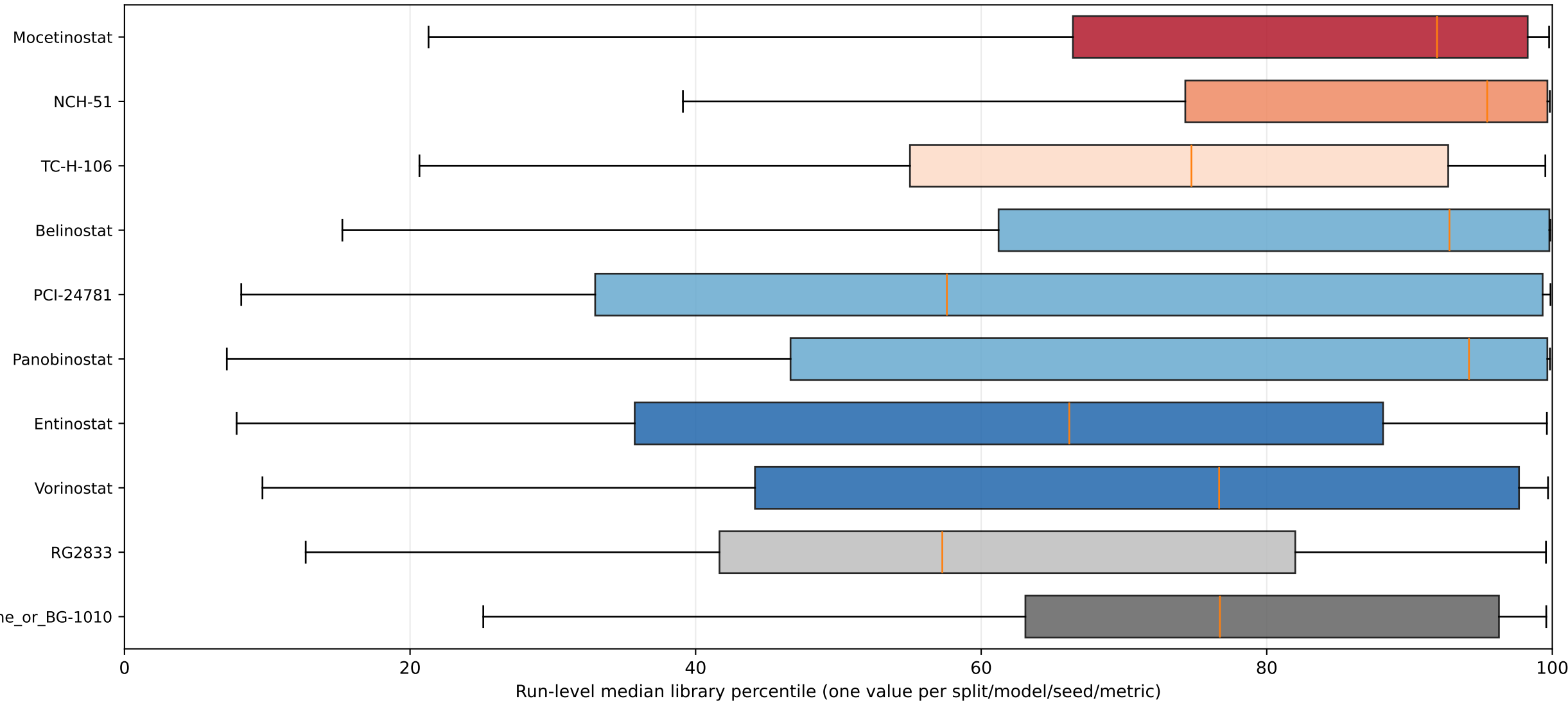
B Distribution across 72 balanced run configurations
