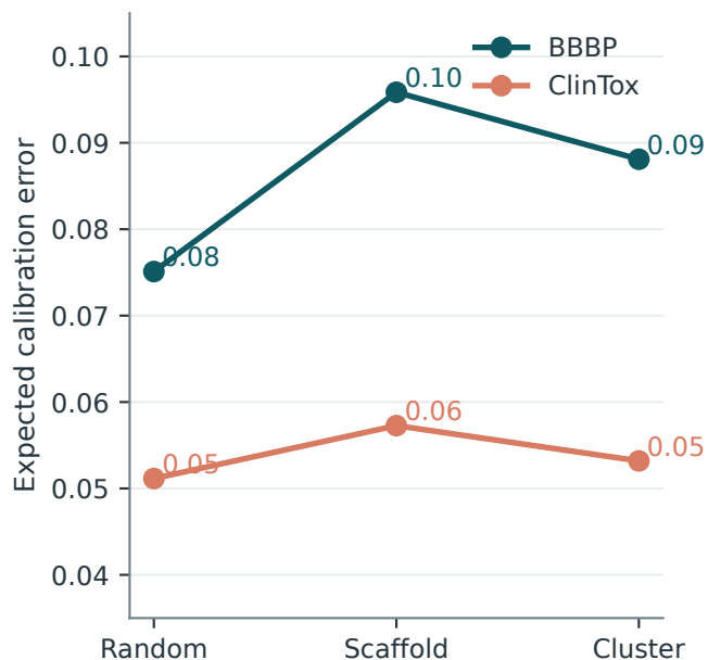
D Positive-probability calibration
