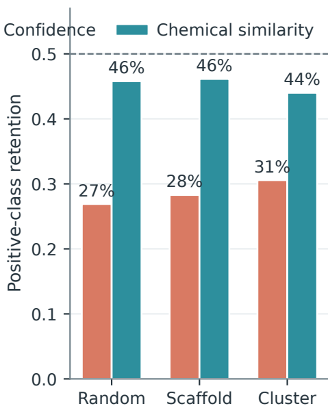
C ClinTox positive retention at 50% coverage
