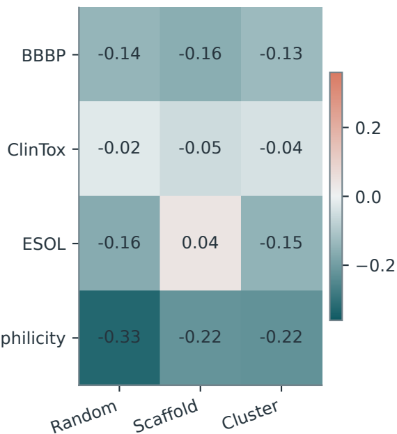
A Similarity versus predictive risk
