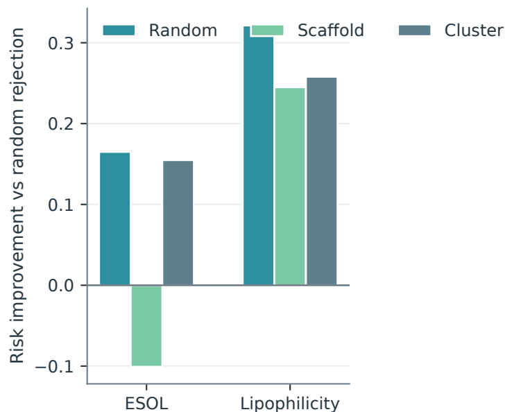
D Regression risk after similarity rejection
