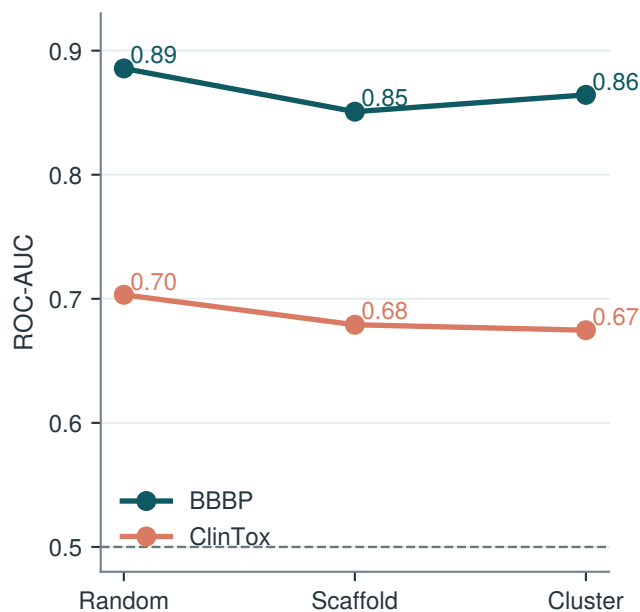
A ROC-AUC under molecular shift
