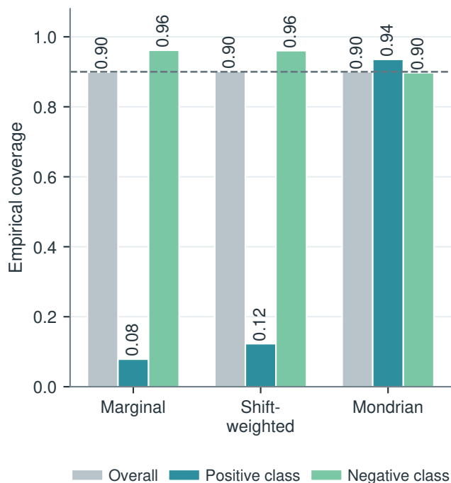
A ClinTox: class-conditional coverage
