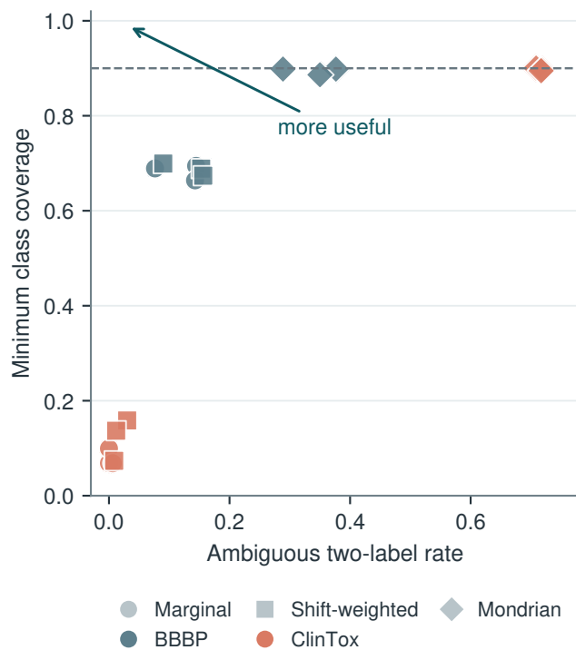
B Coverage-ambiguity trade-off
