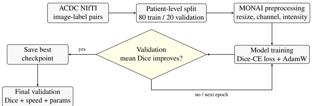
Figure 5.1: Reproducible experimental workflow. The main methodological safeguard is patient-level separation before training, so that validation cases come from patients not seen during optimization.
