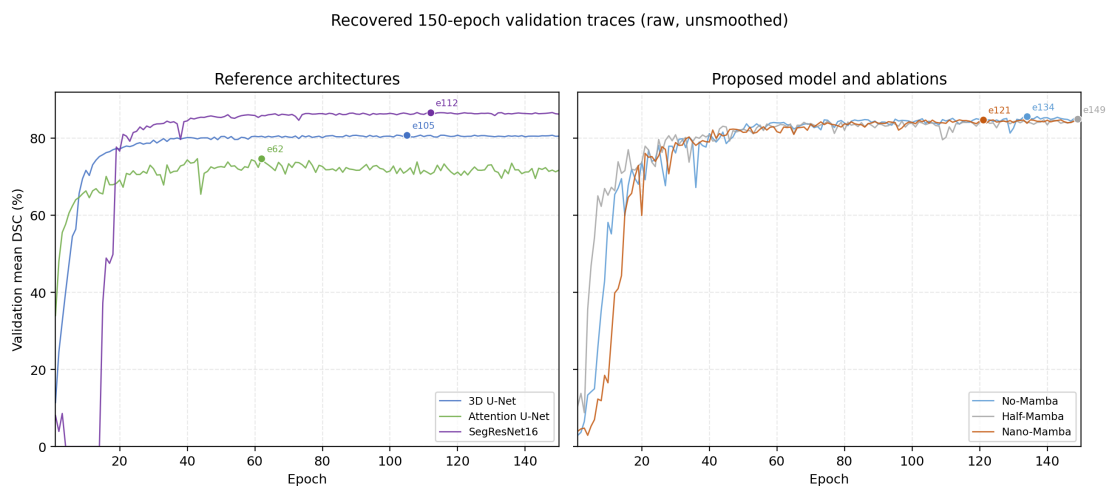
Figure 6.4: Recovered raw, unsmoothed 150-epoch validation mean-DSC traces. Markers identify the best validation checkpoint selected for each model. The figure is generated directly from the six byte-hashed training-log CSVs.
