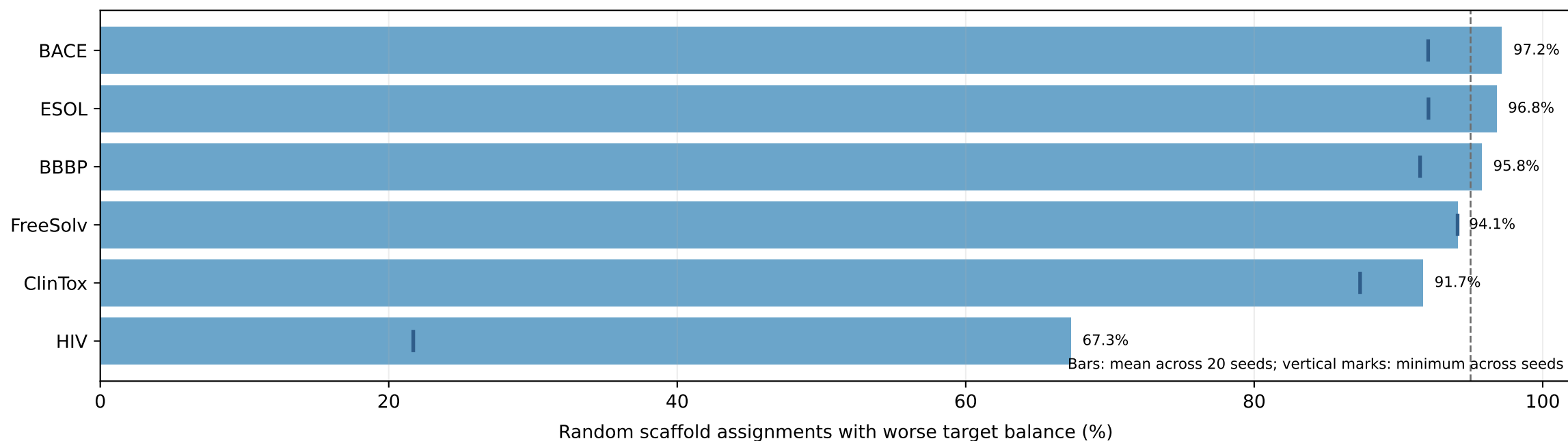
A Target-balanced scaffold assignments relative to the random-scaffold null
