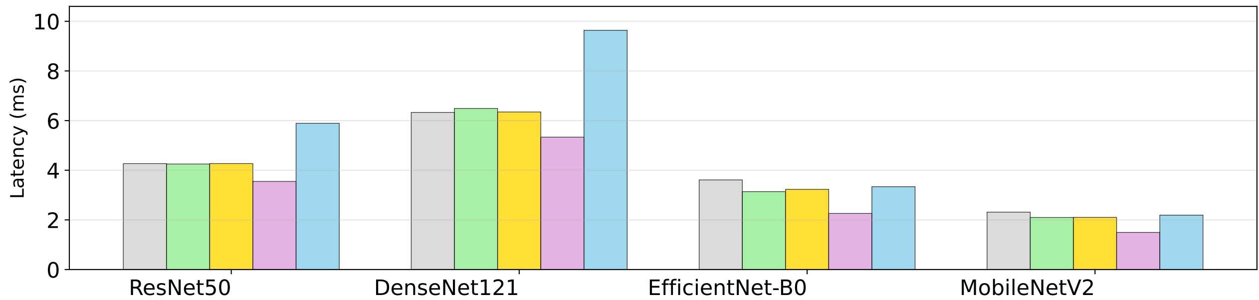
Batch Size 8
