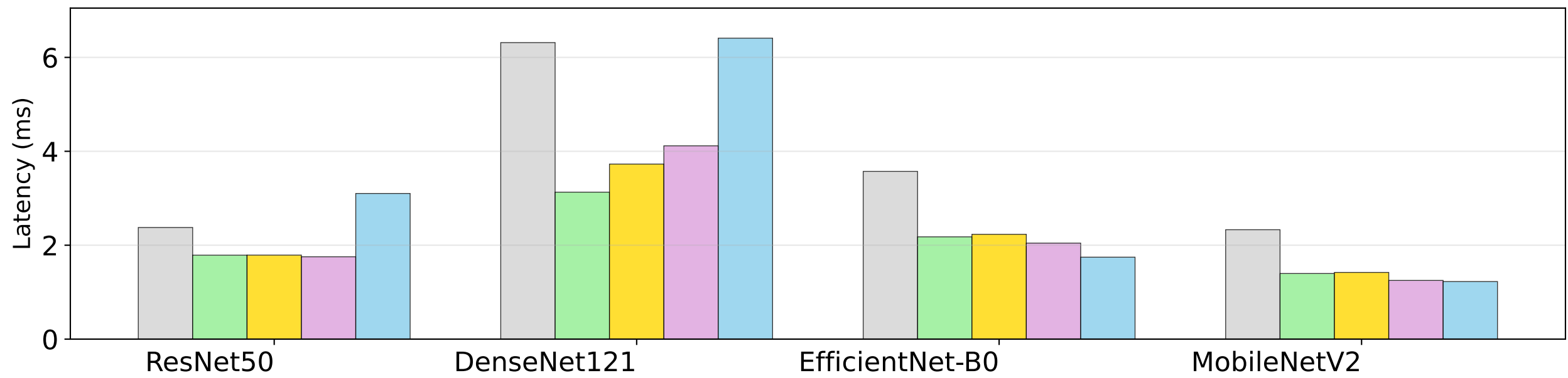
Batch Size 1
