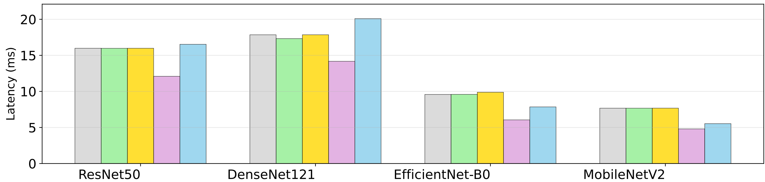
Batch Size 32
