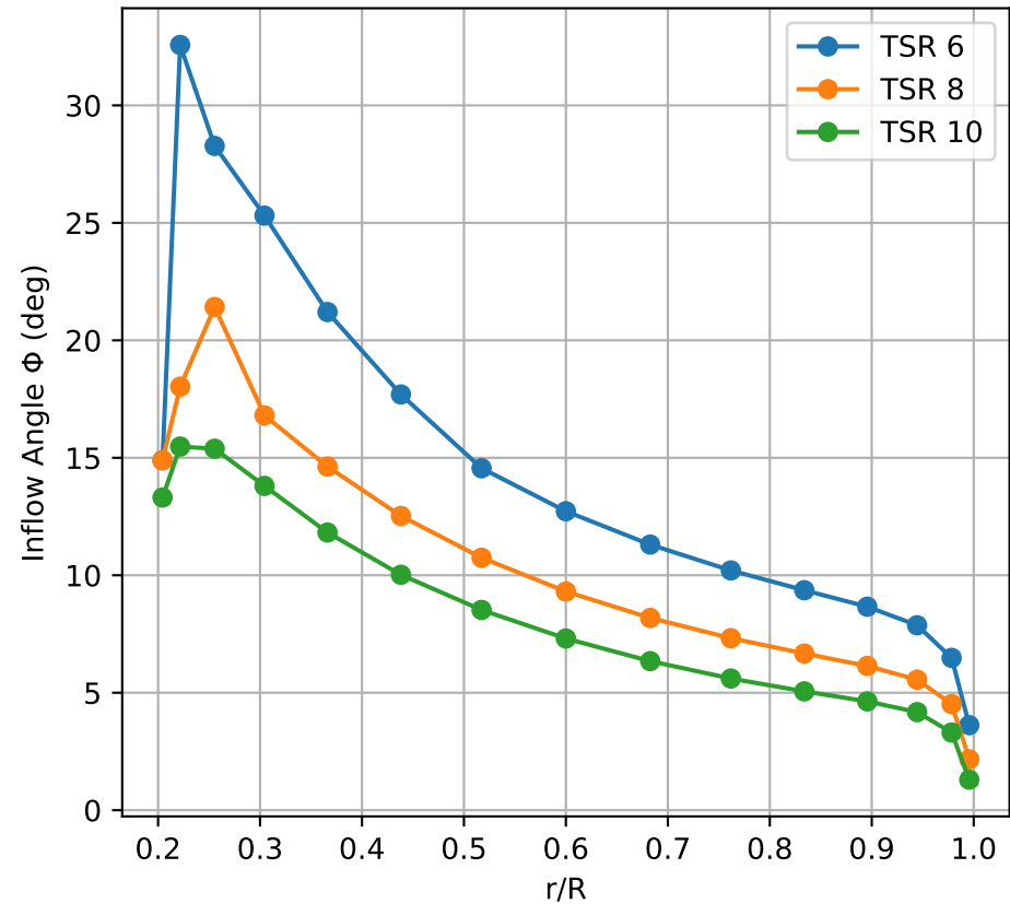
Radial Distribution of Inflow Angle
