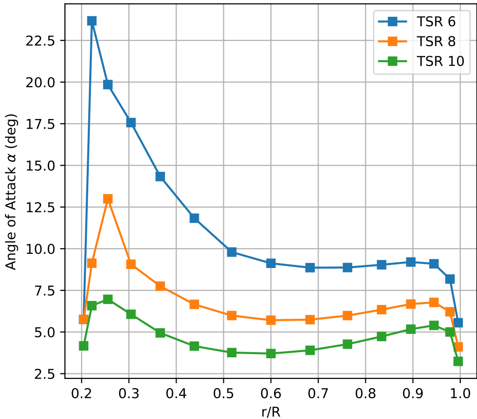
Radial Distribution of Angle of Attack
