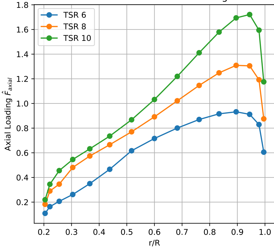
Non-dimensional Axial Loading
