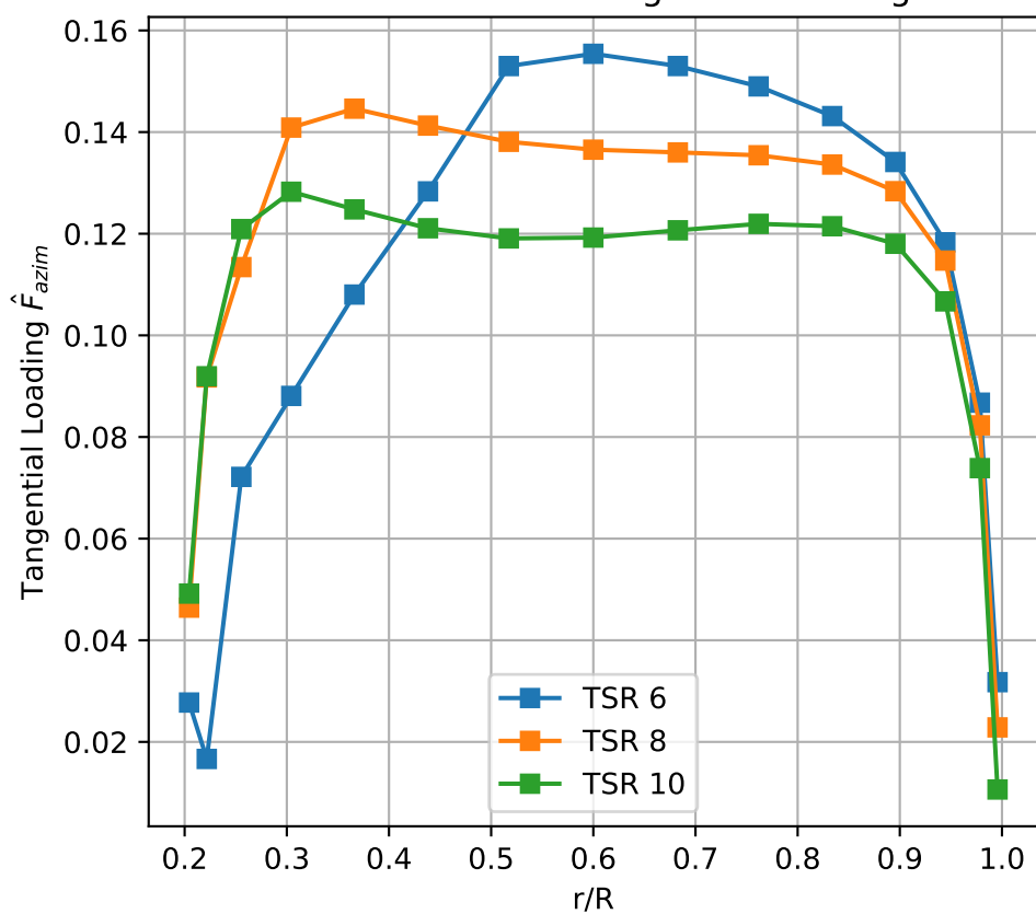
Non-dimensional Tangential Loading
