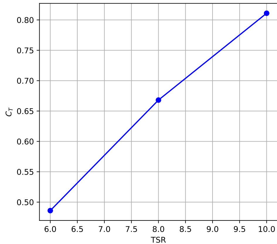
Total Thrust Coefficient
