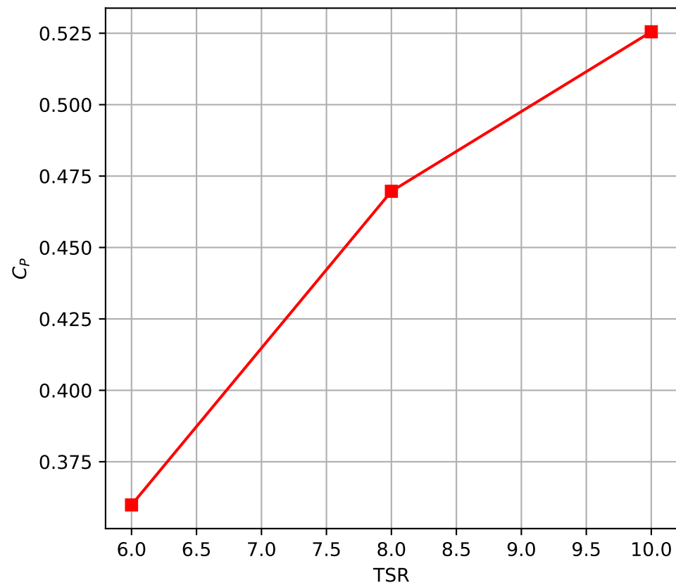
Total Power Coefficient
