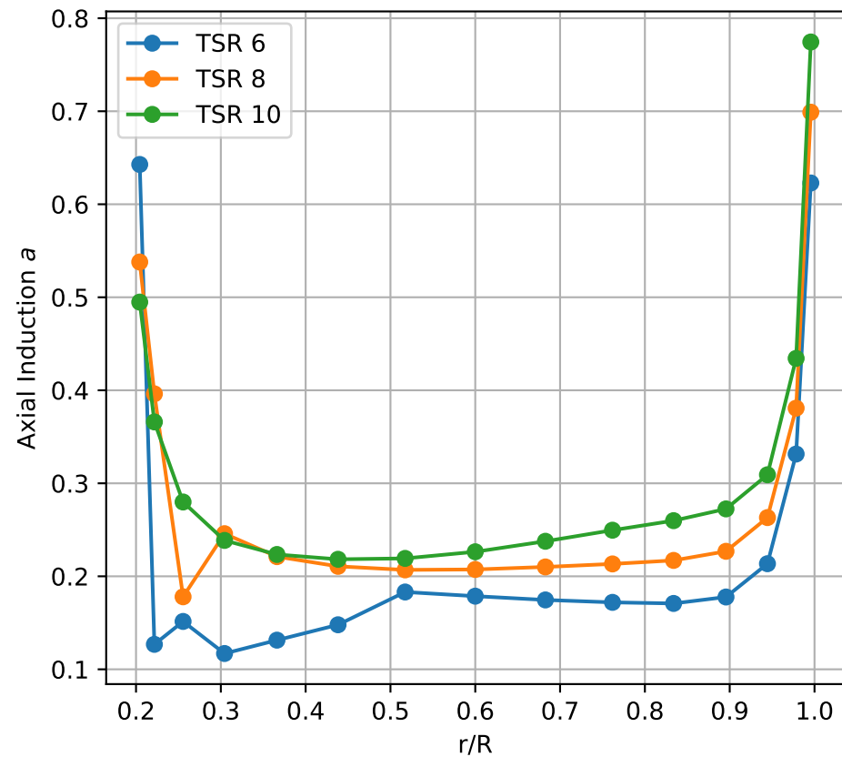
Radial Distribution of Axial Induction
