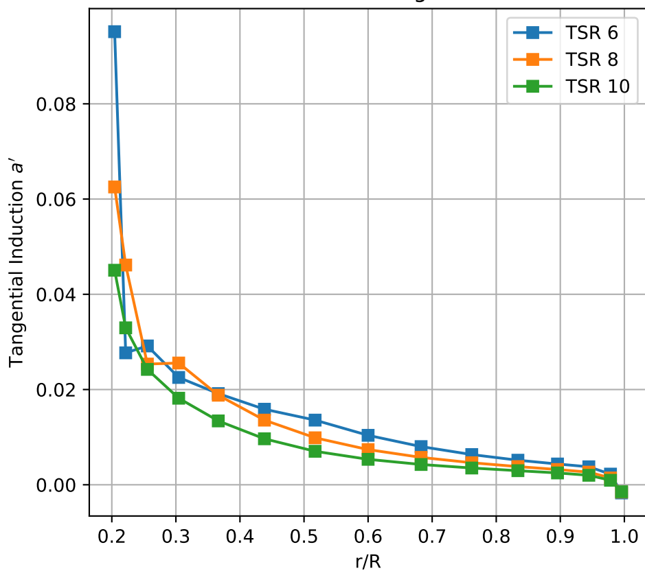
Radial Distribution of Tangential Induction
