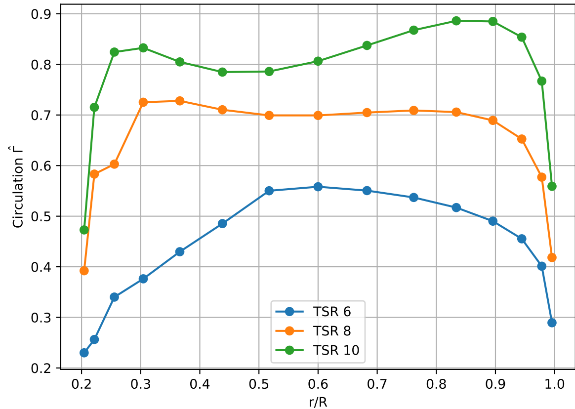
Non-dimensional Radial Circulation
