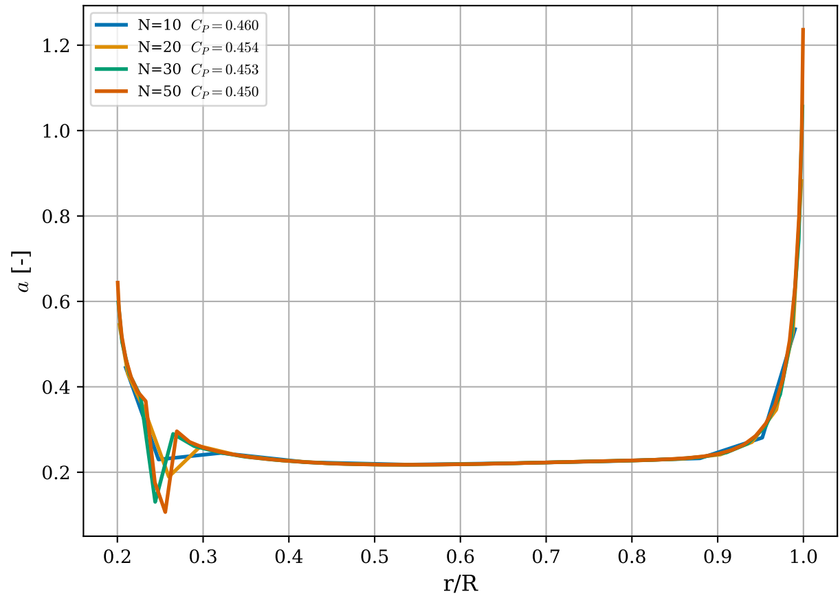
Axial induction (cosine)
