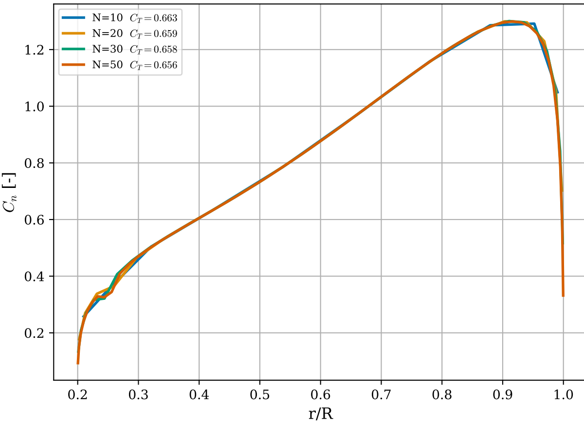
Panel count sensitivity (cosine)
