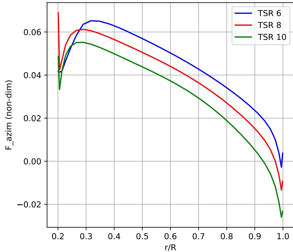
Tangential Loading
