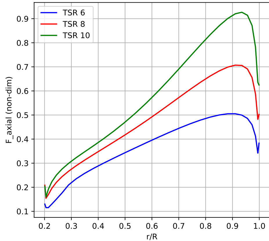
Axial Loading
