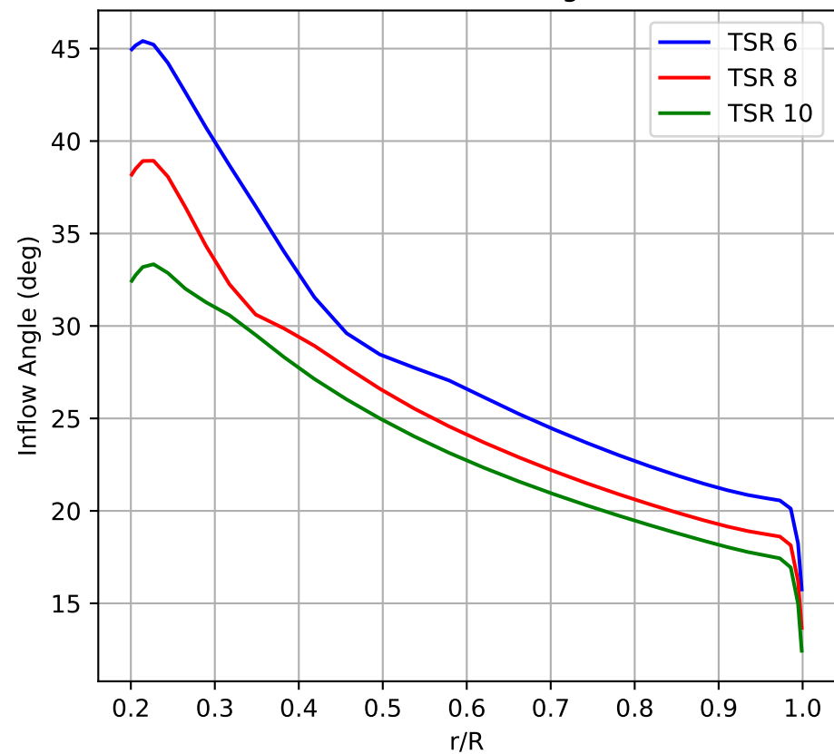
Radial Inflow Angle
