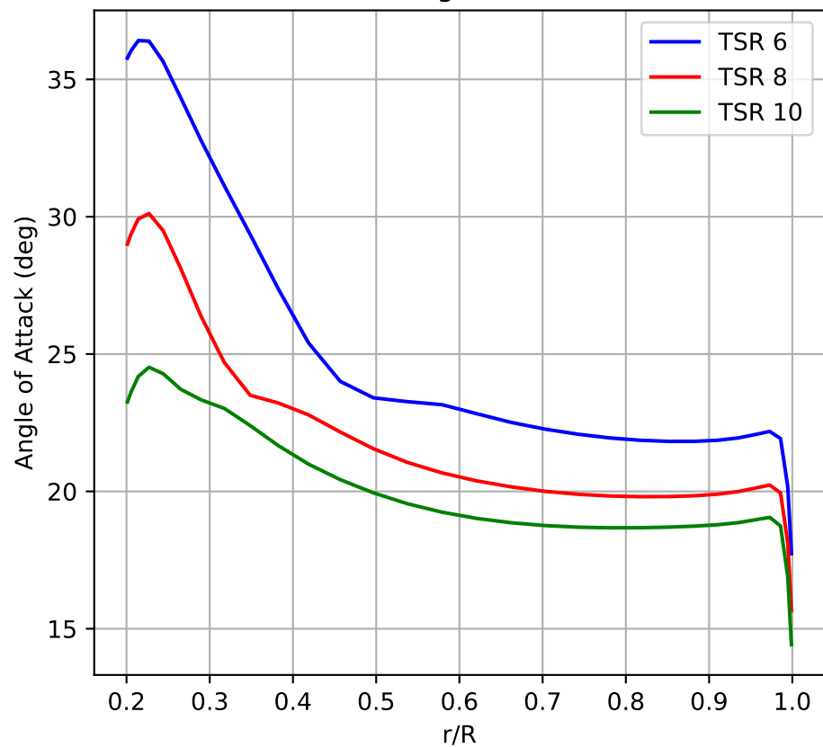
Radial Angle of Attack
