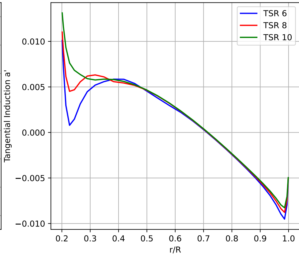
Tangential Induction
