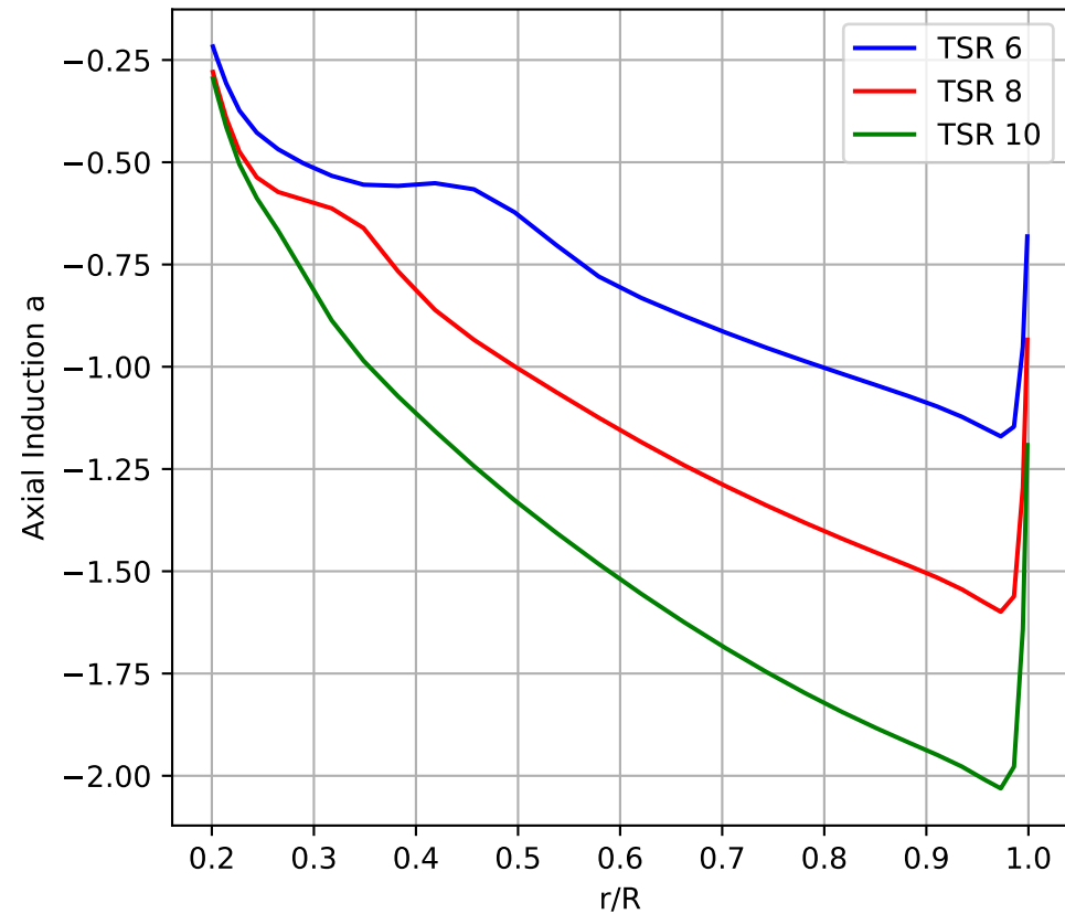
Axial Induction
