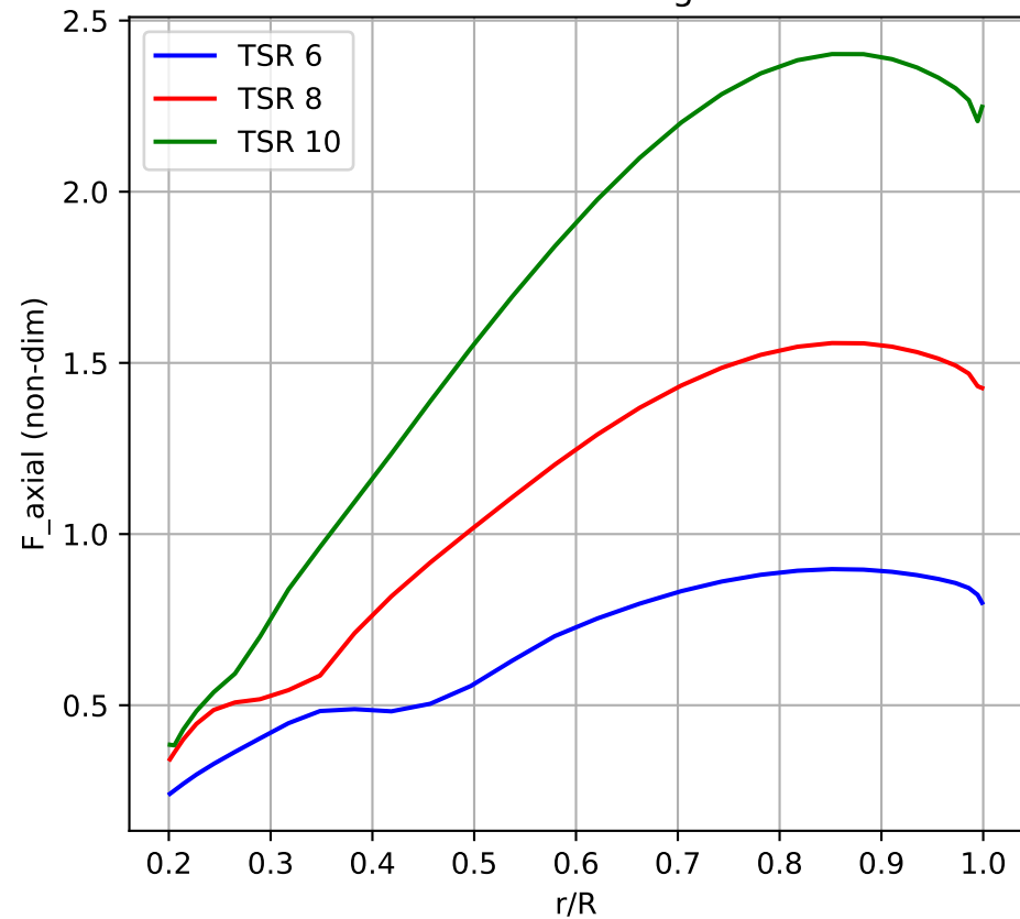
Axial Loading
