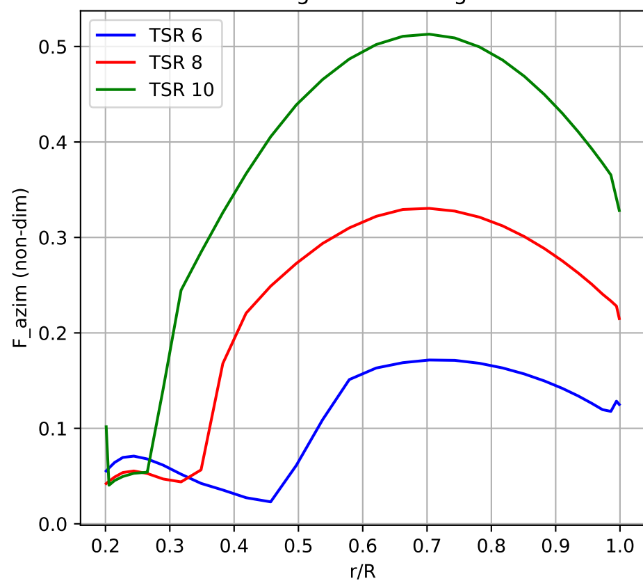
Tangential Loading
