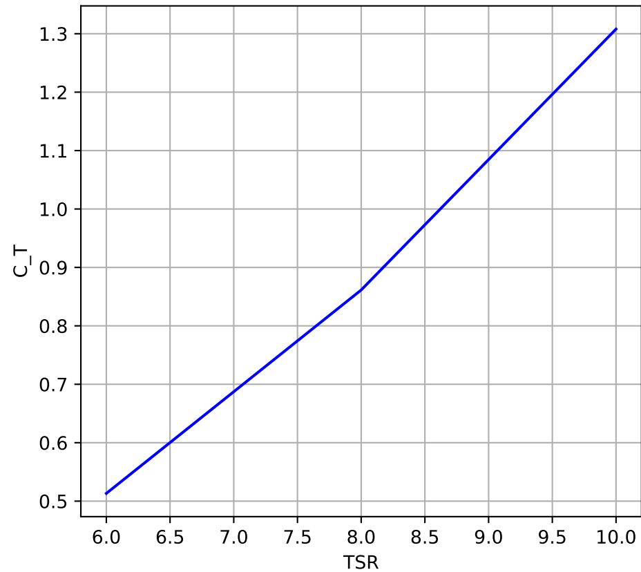
Thrust Coefficient
