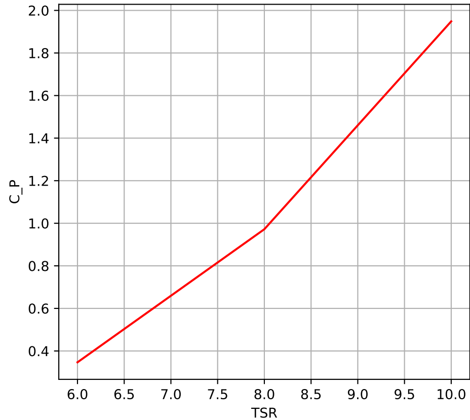
Power Coefficient
