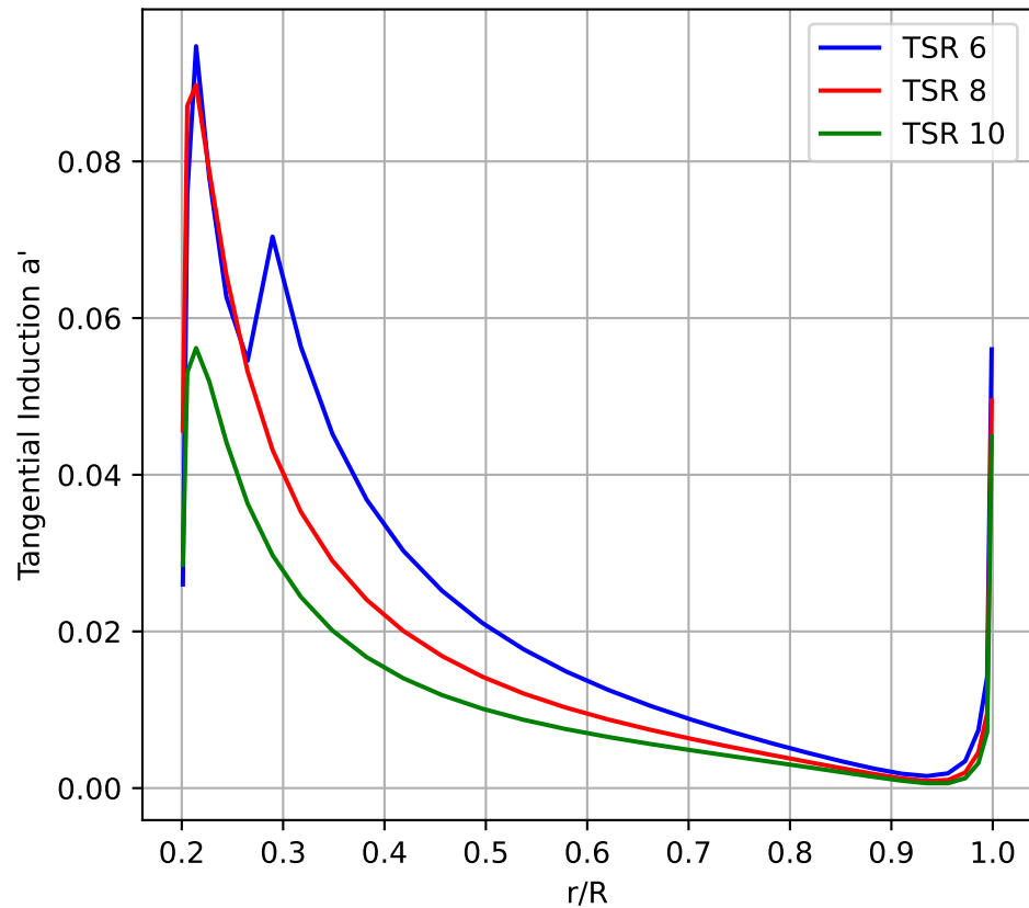
Tangential Induction
