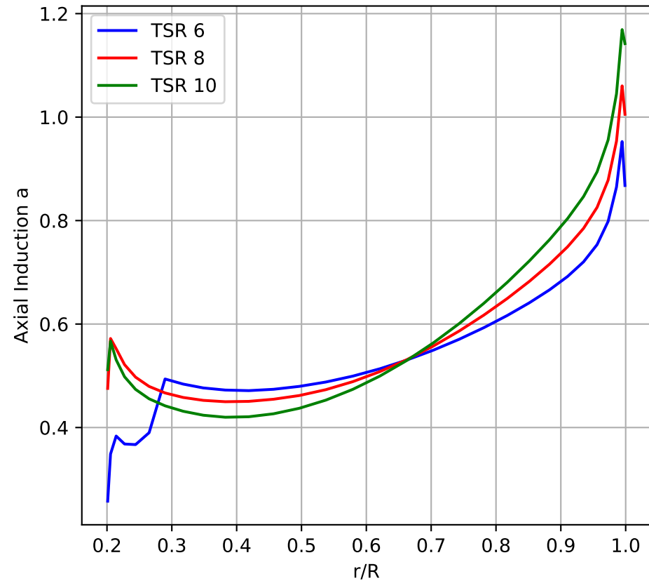
Axial Induction
