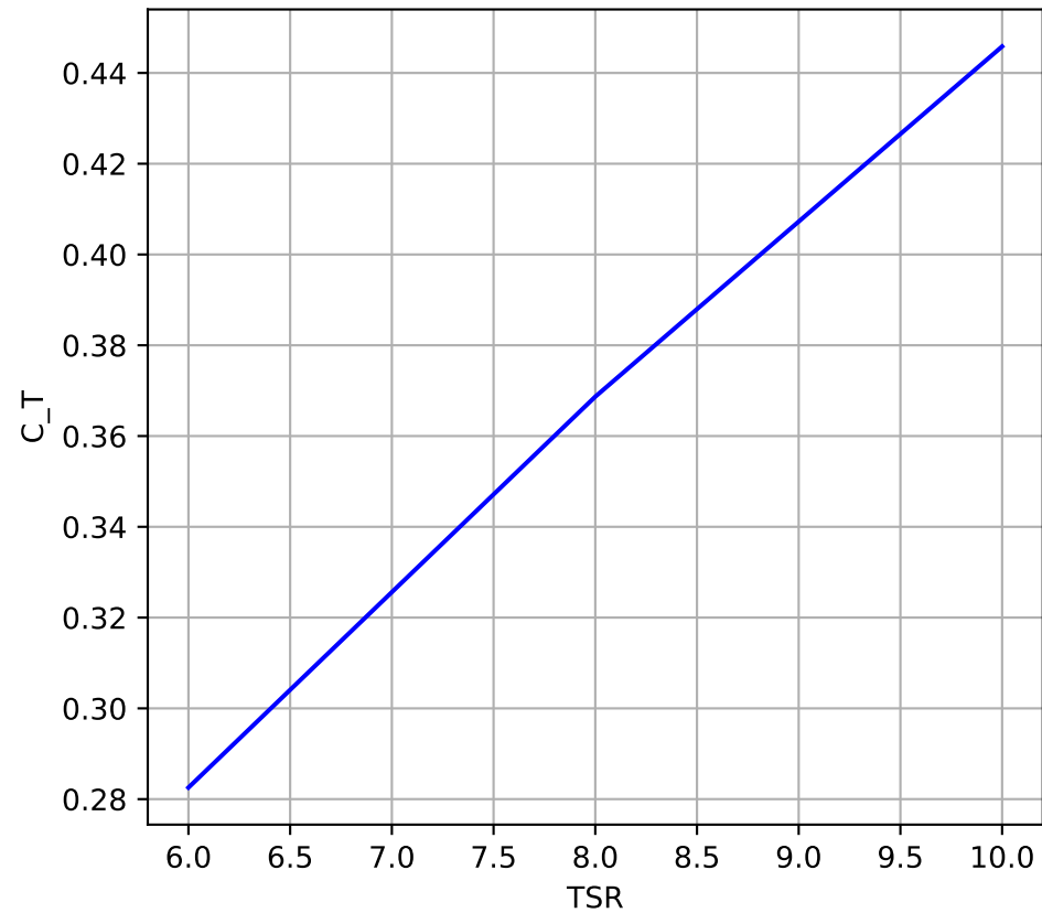
Thrust Coefficient
