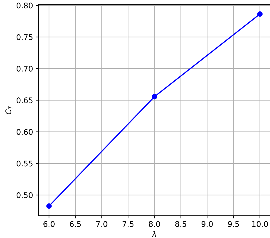
Thrust Coefficient
