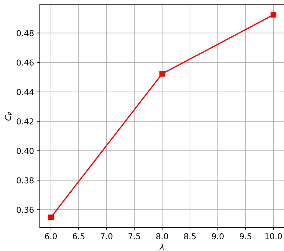
Power Coefficient
