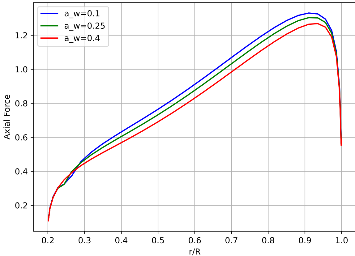
Sensitivity: Convection Speed ( a_w )
