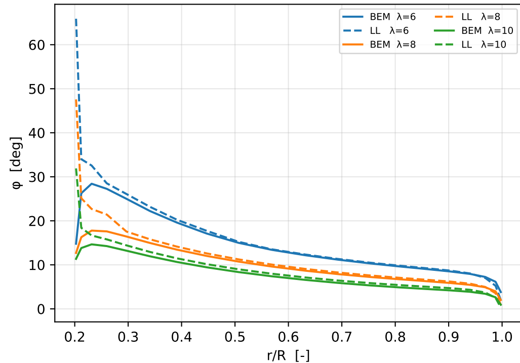
Inflow angle \varphi
