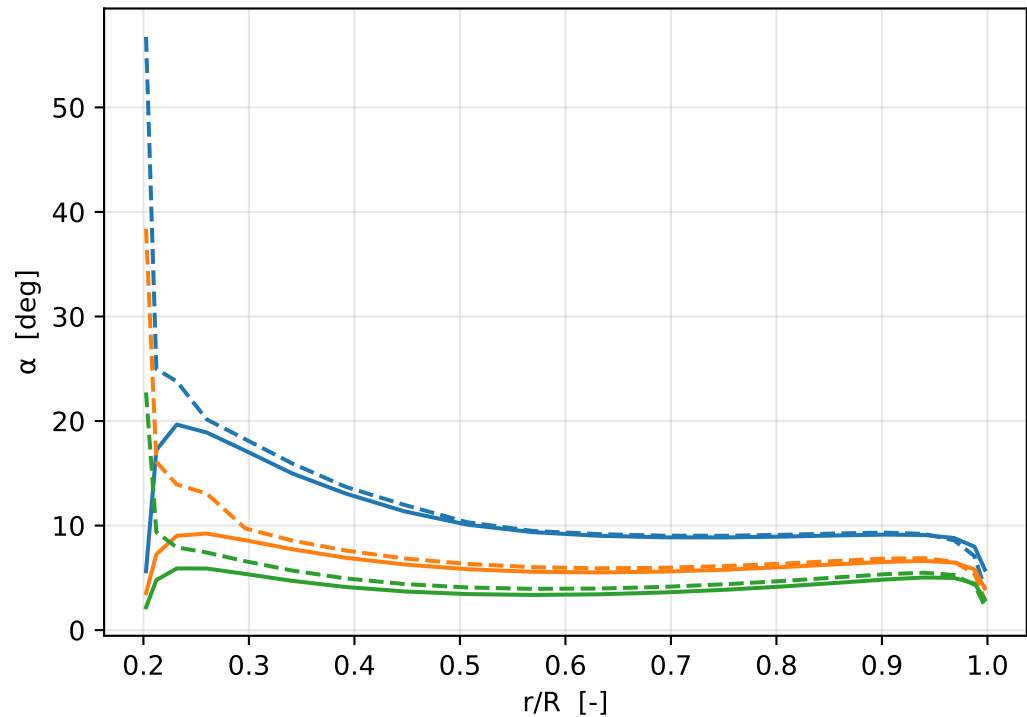
Angle of attack \alpha
