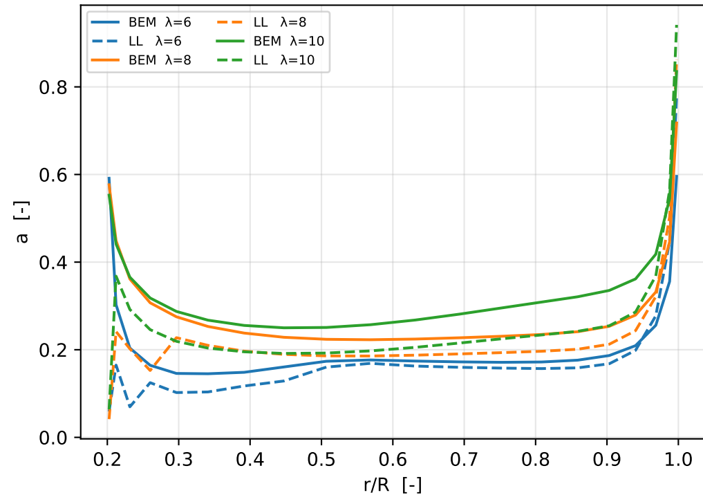
Axial induction a
