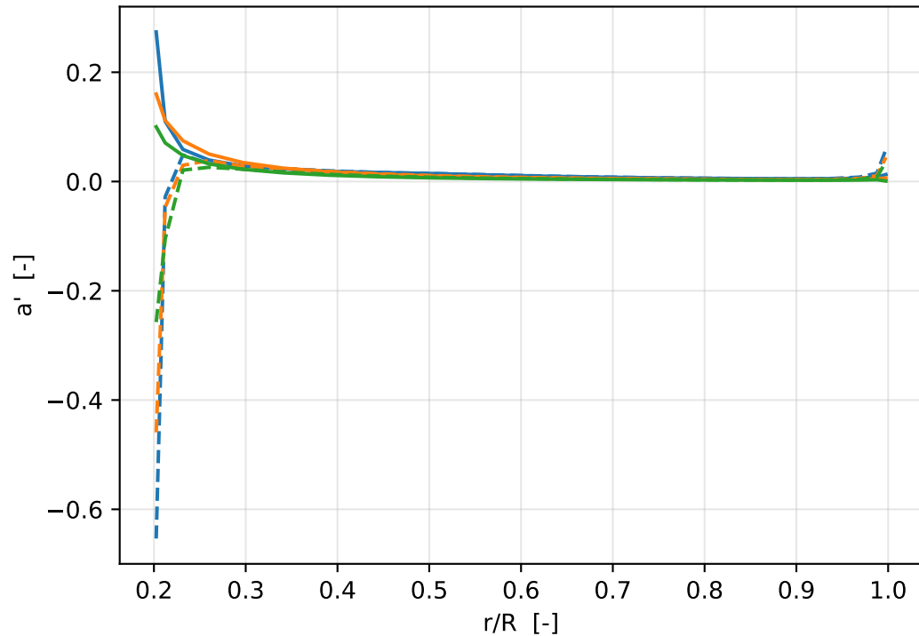
Tangential induction a'
