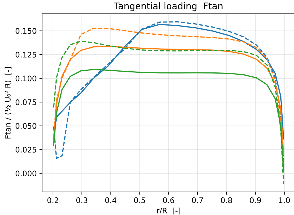
Radial distribution — non-dimensional blade loading
