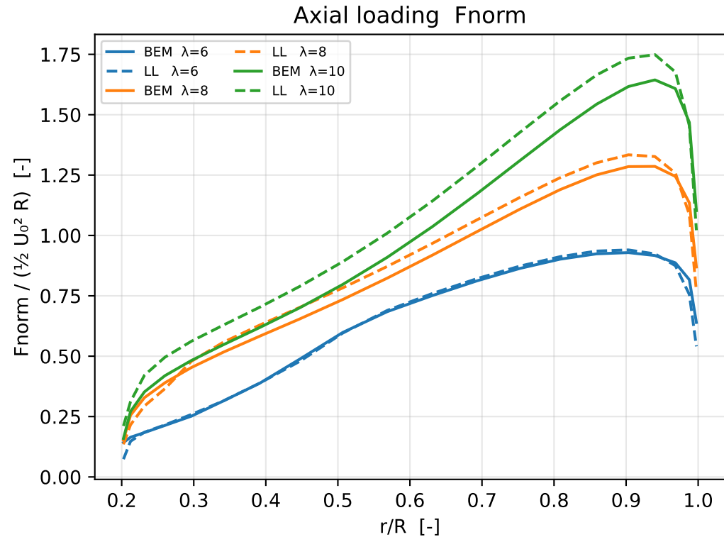
Radial distribution — non-dimensional blade loading
