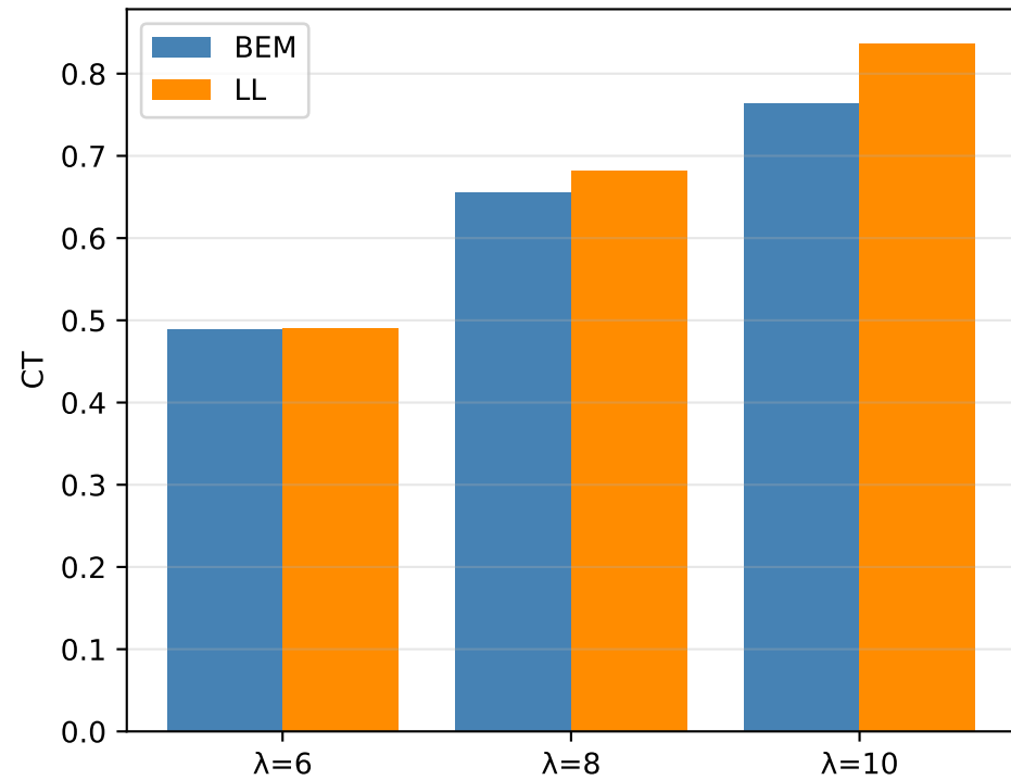
Thrust coeff. CT
