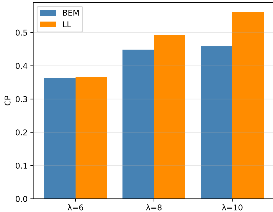
Power coeff. CP
