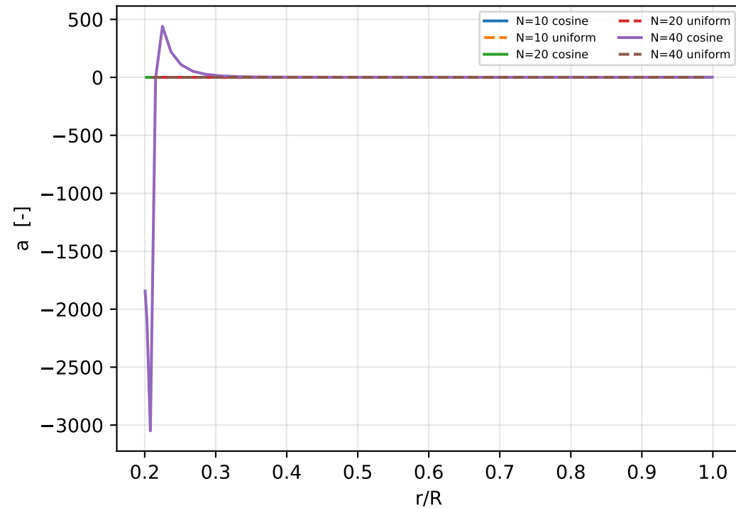
Axial induction
