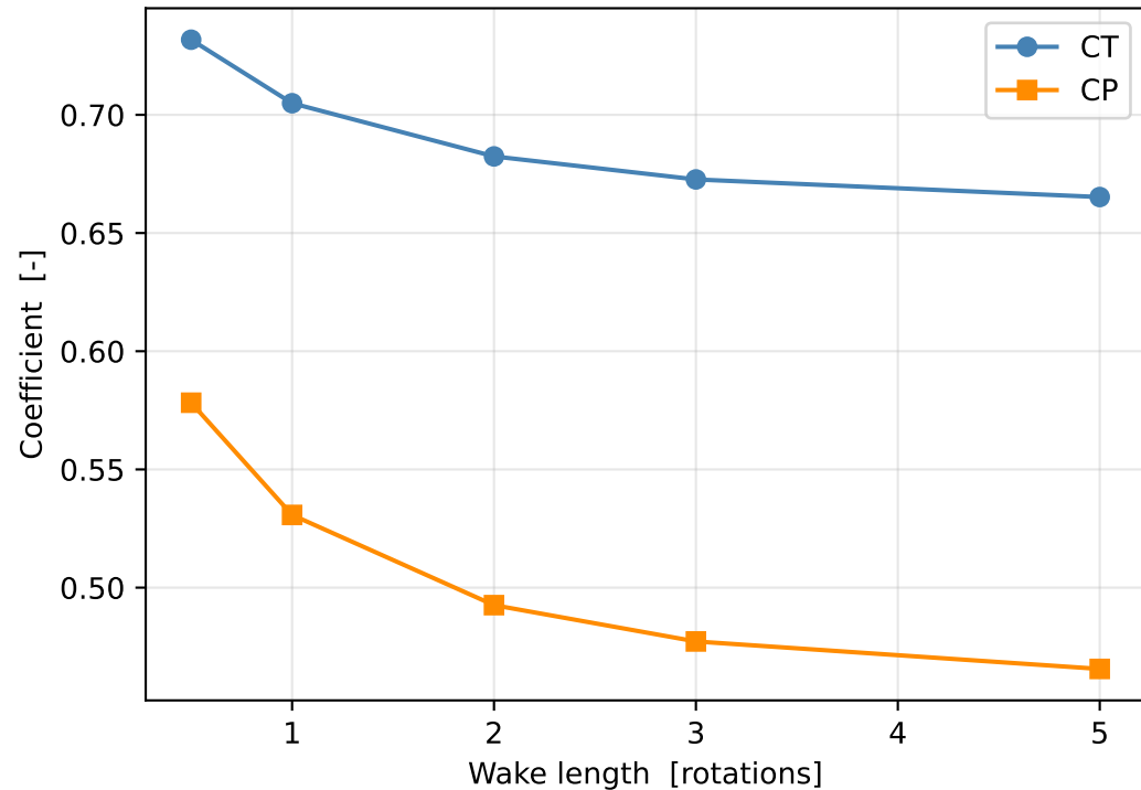
CT and CP convergence with wake length
