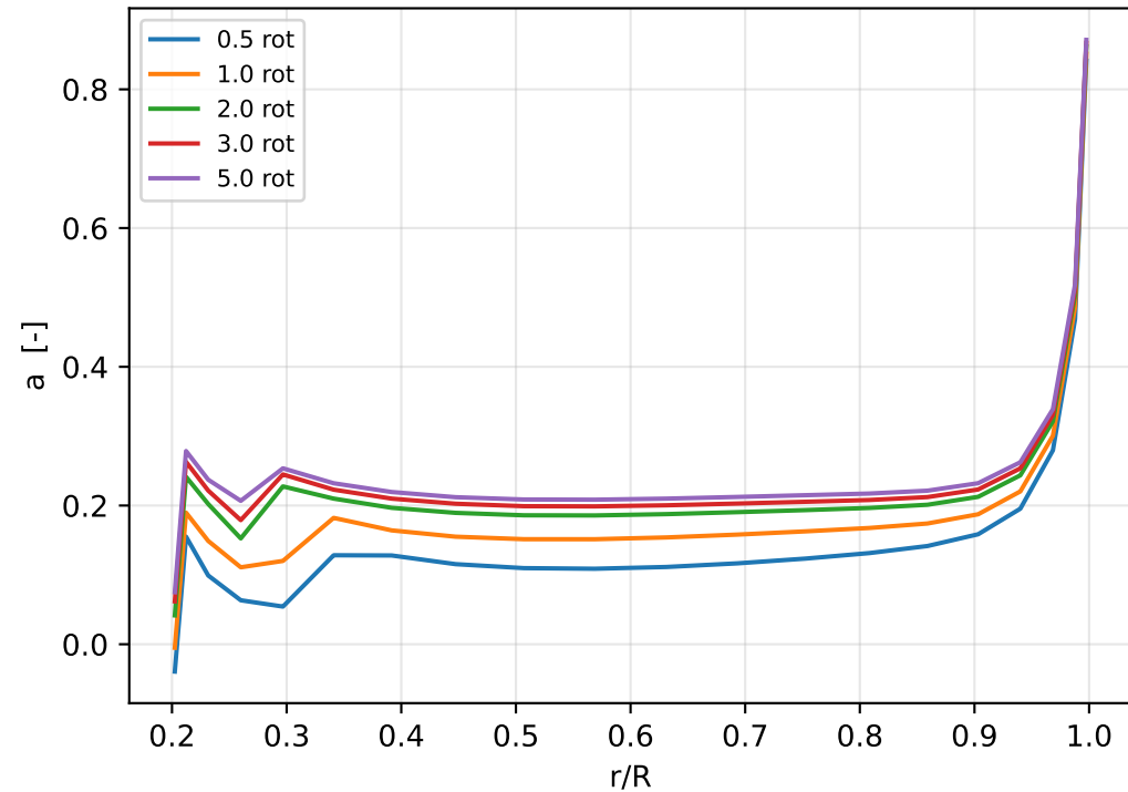
Axial induction
