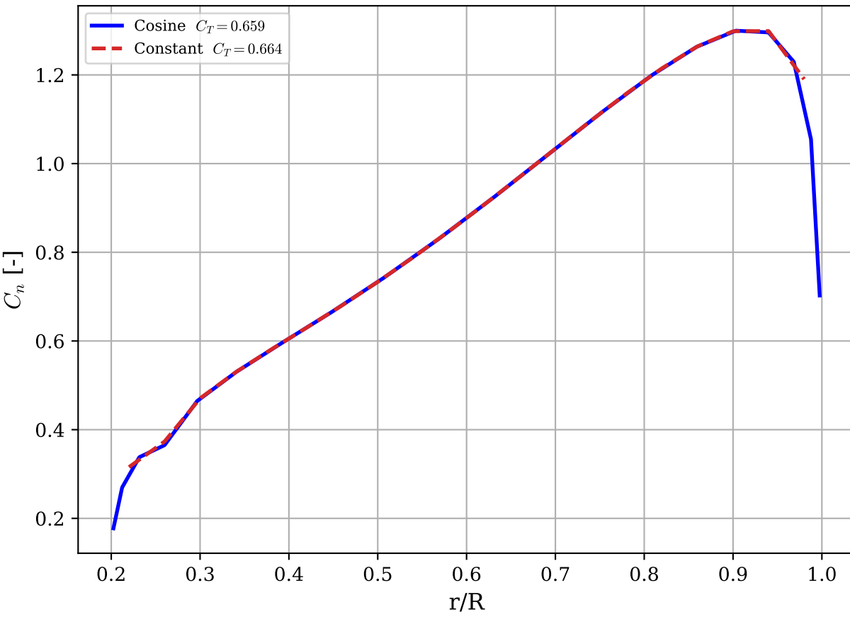
Cosine vs constant spacing (N=20)
