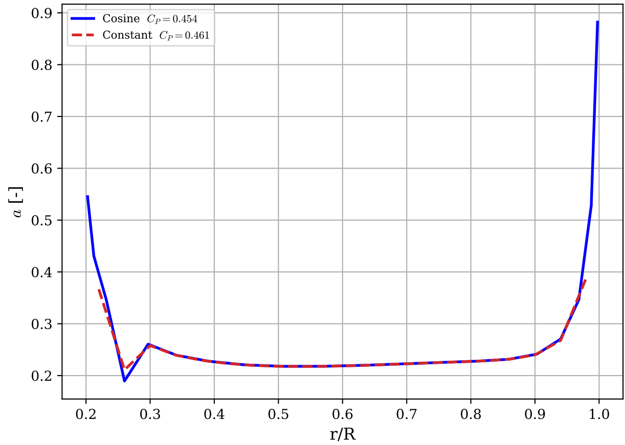
Axial induction (N=20)
