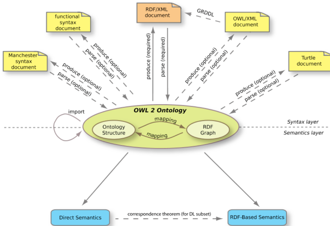
Figure 2.4: The OWL2 Structure [100].
