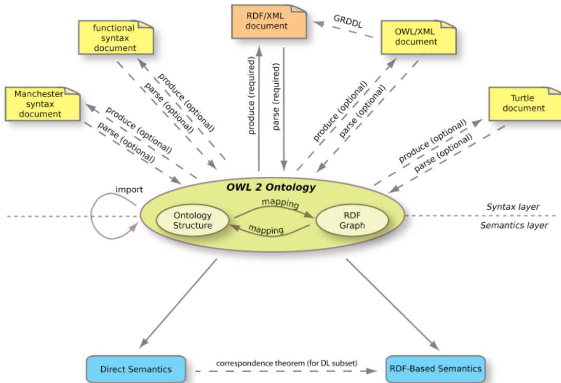
Figure 2.2: The OWL2 Structure [86].
