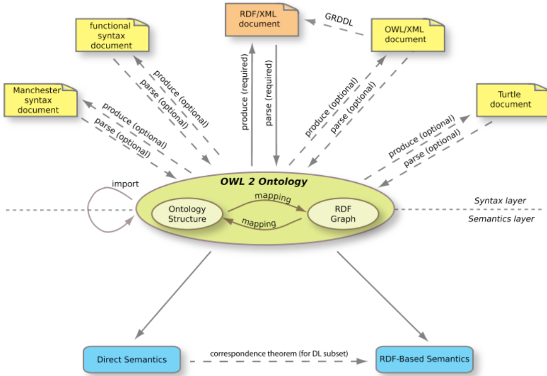
Figure 2.2: The OWL2 Structure [47].
