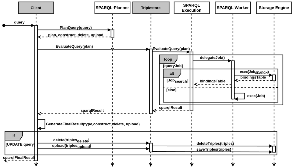
Figure 3.1: SPARQL-EVAL Sequence Diagram (query evaluation).
