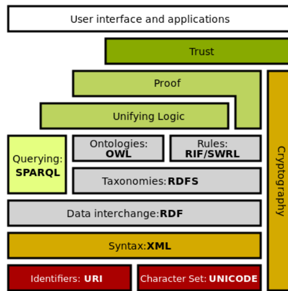
Figure 2.1: The Semantic Web stack [33]
