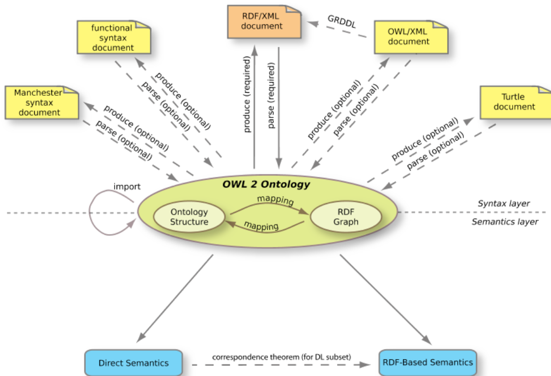
Figure 2.4: The OWL2 Structure [97].
