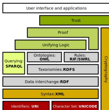
Figure 2.1: The Semantic Web stack [116].
