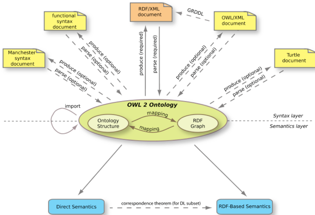
Figure 2.2: The OWL2 Structure [74].
