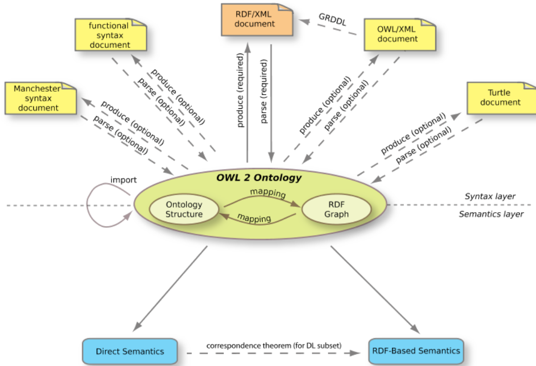
Figure 2.4: The OWL2 Structure [88].
