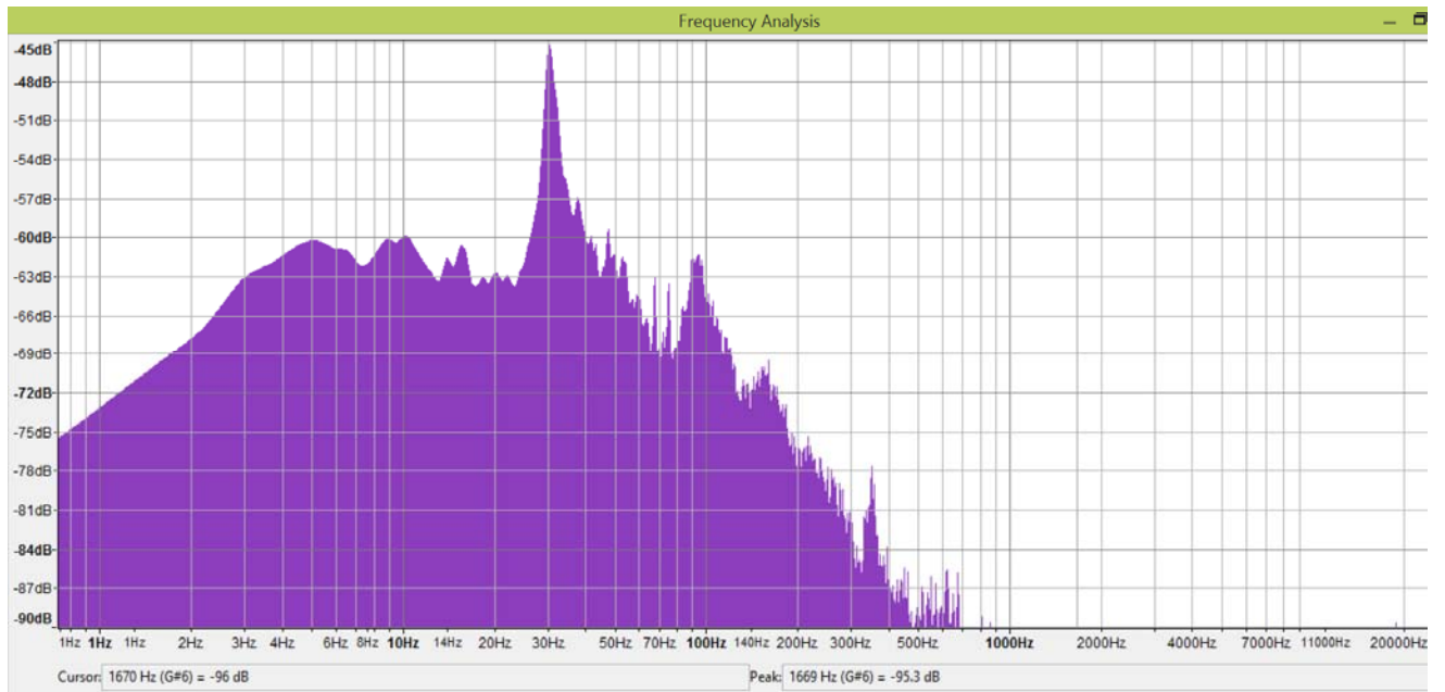
„silence“ Stereo-recording 48ksps, two I2S mics ICS43434
