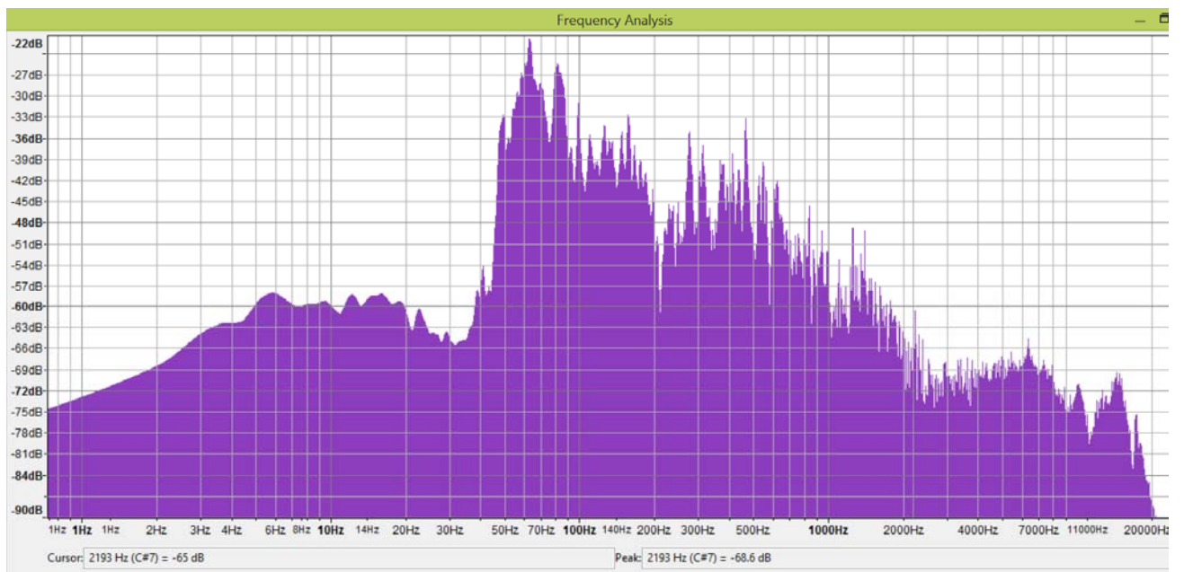
“music” Stereo-recording 48ksps, two I2S mics ICS43434
