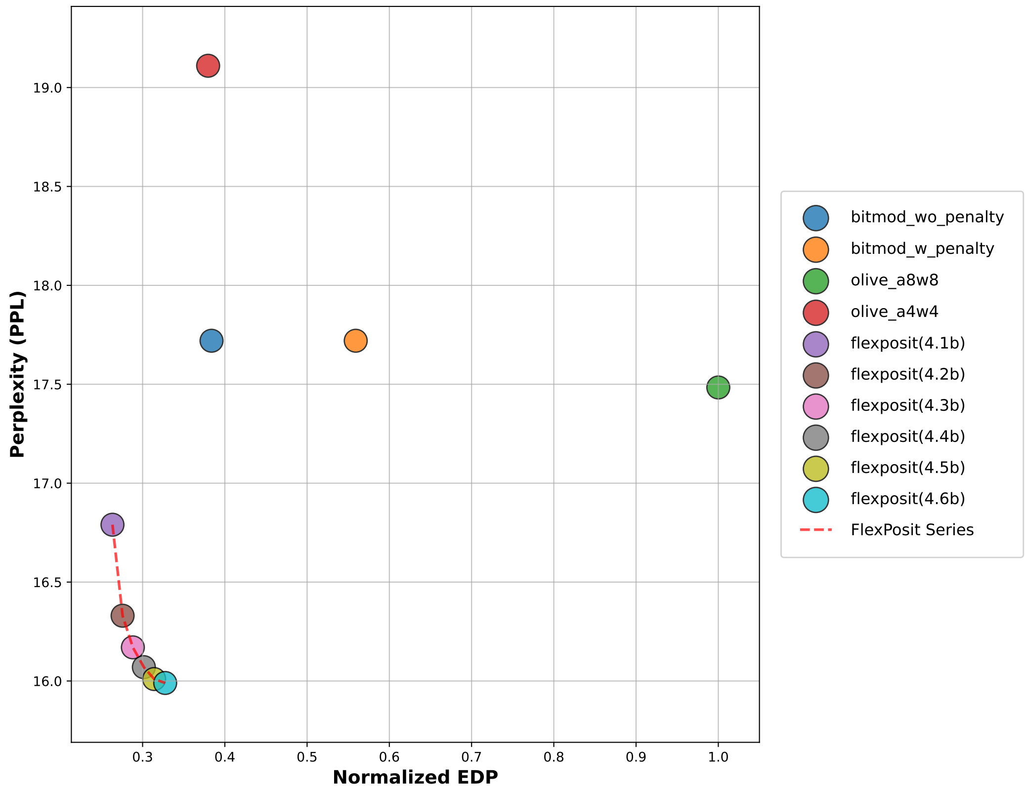
PPL vs Normalized EDP (gpt2-xl)
