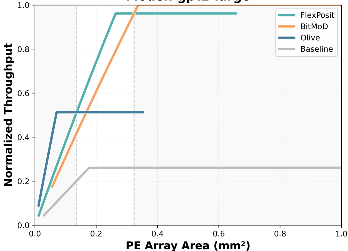
Model: gpt2-large
