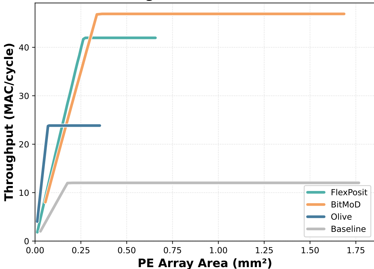
Average over Models (Raw)
