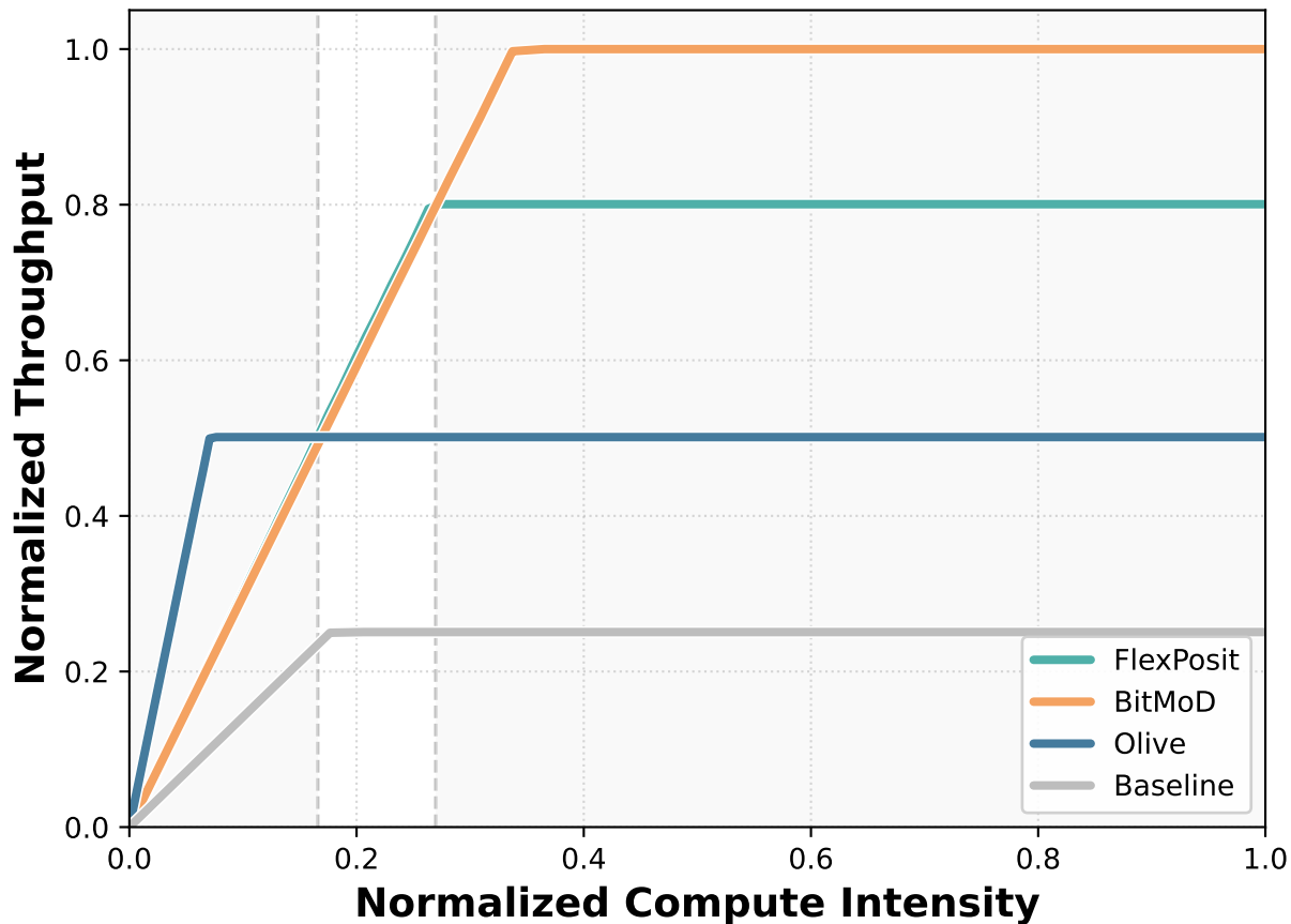
Model: meta-llama/Llama-2-7b-hf
