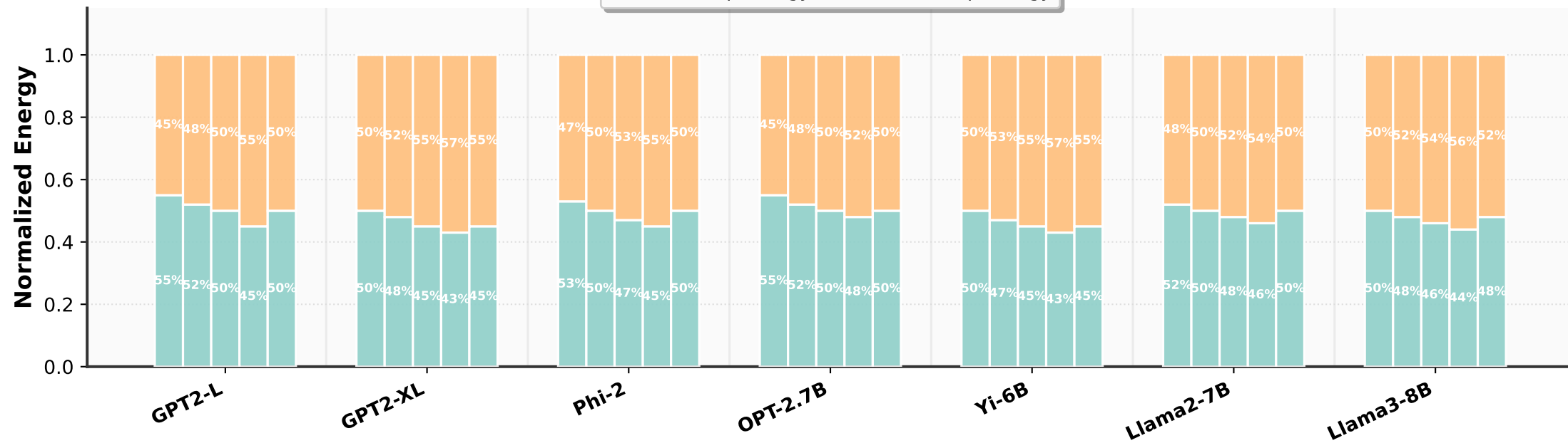
(b) Energy Consumption Breakdown
