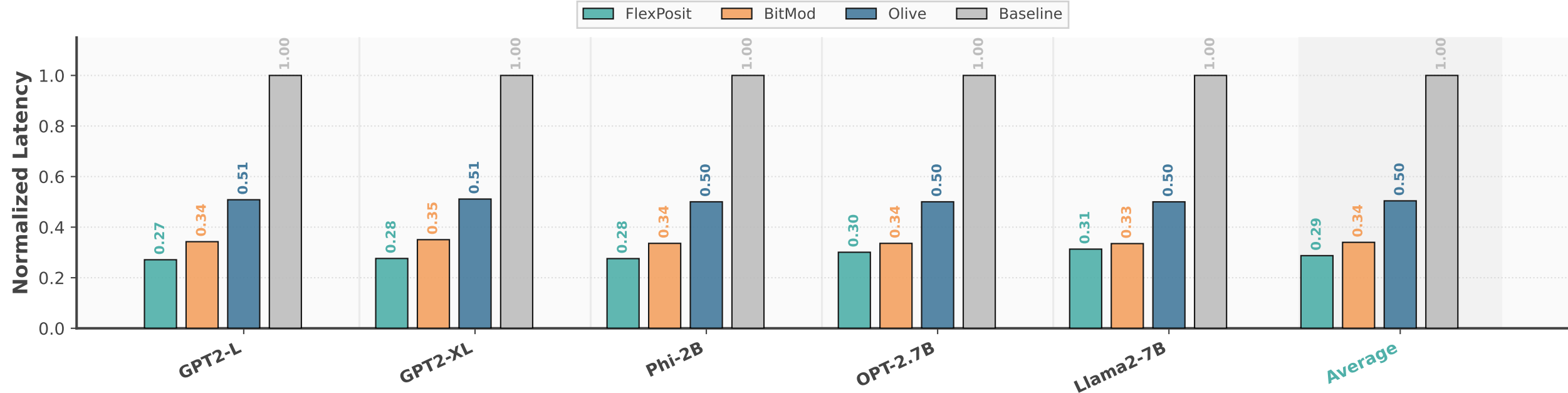
(a) Inference Latency Comparison
