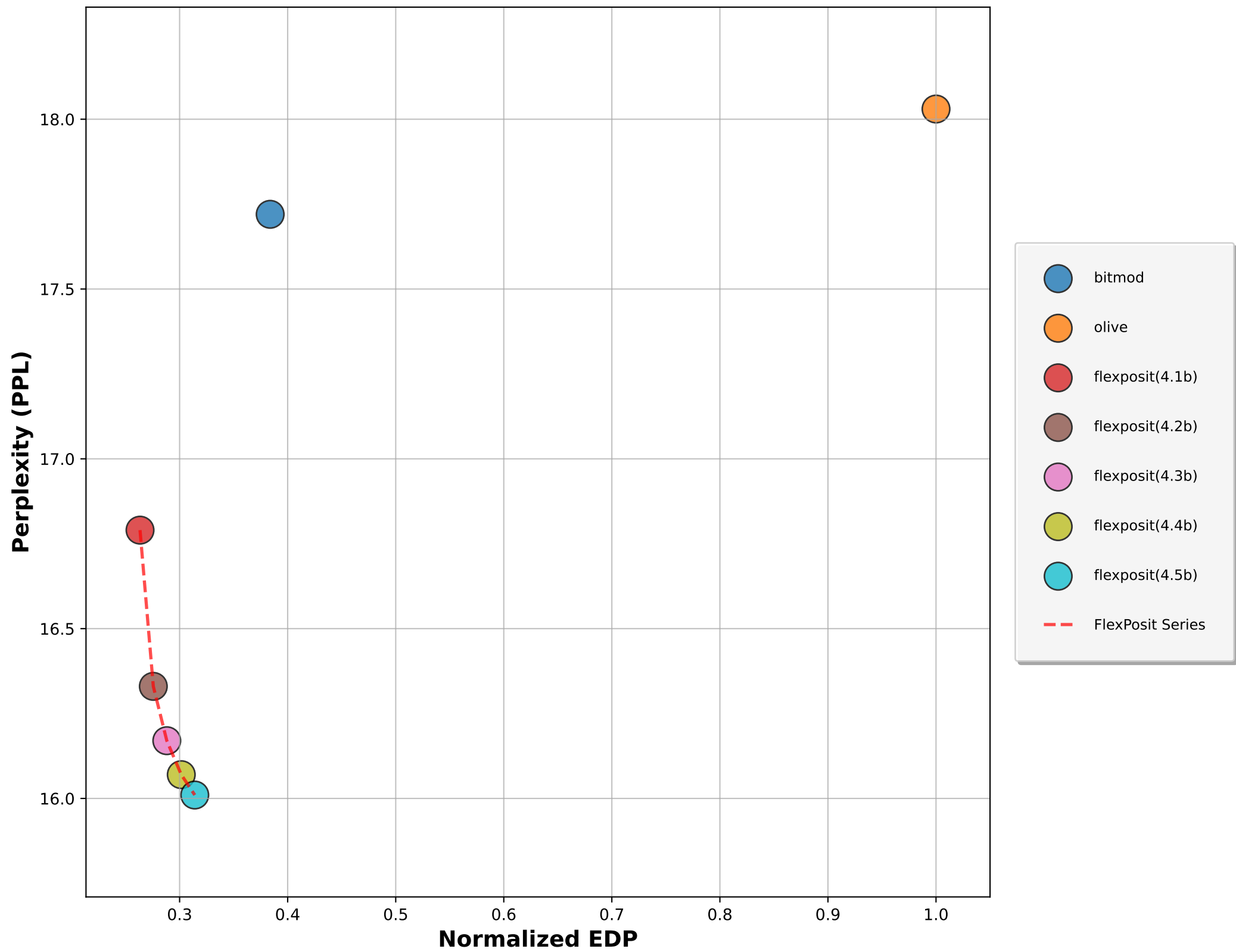
PPL vs Normalized EDP Scatter Plot (GPT-2 XL)
