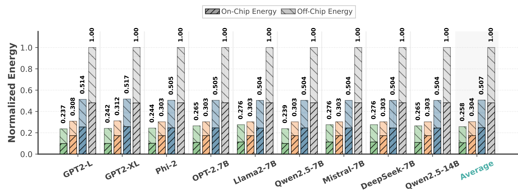
(b) Normalized Energy
